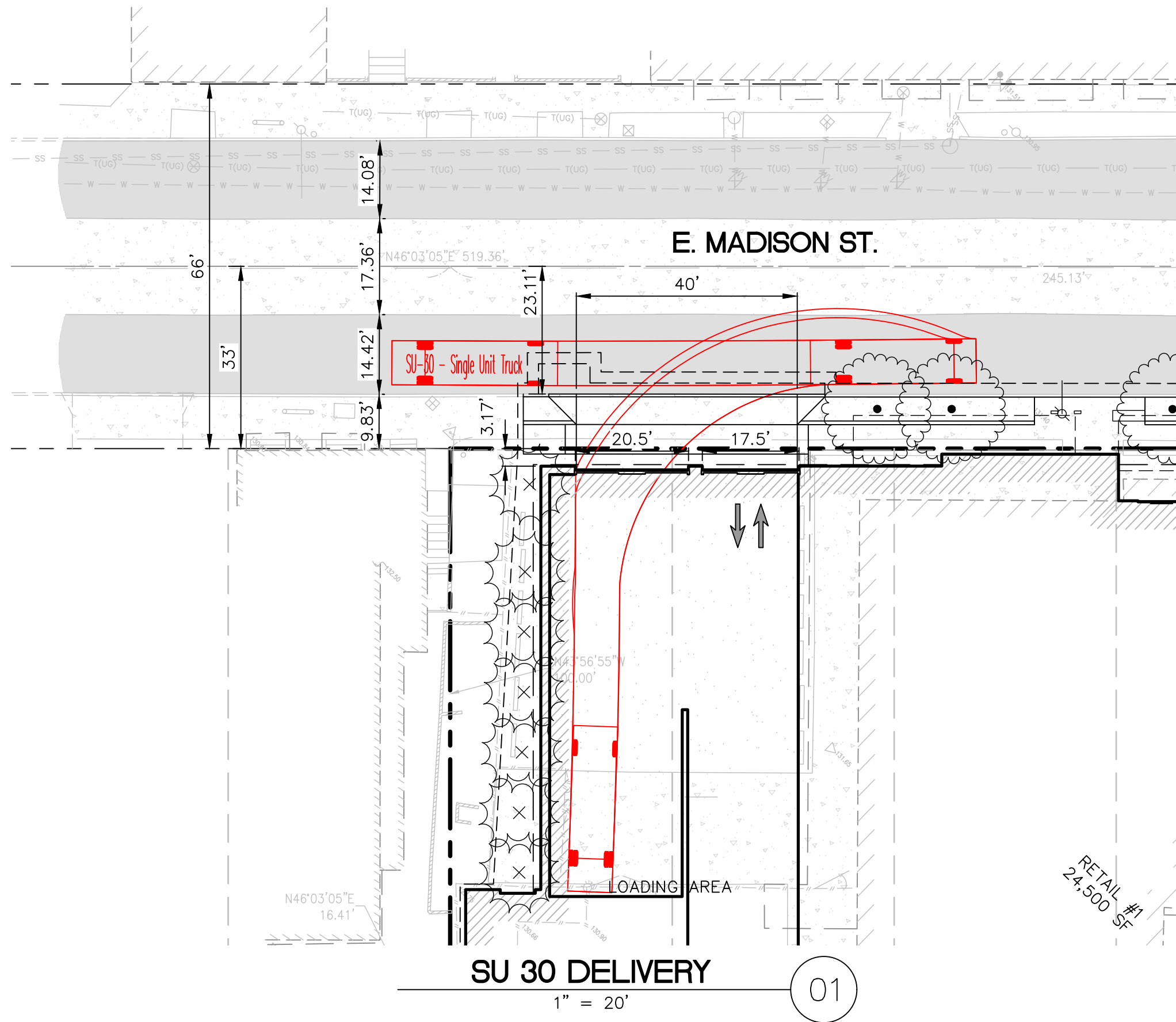
SU-30 - Single Unit Truck
