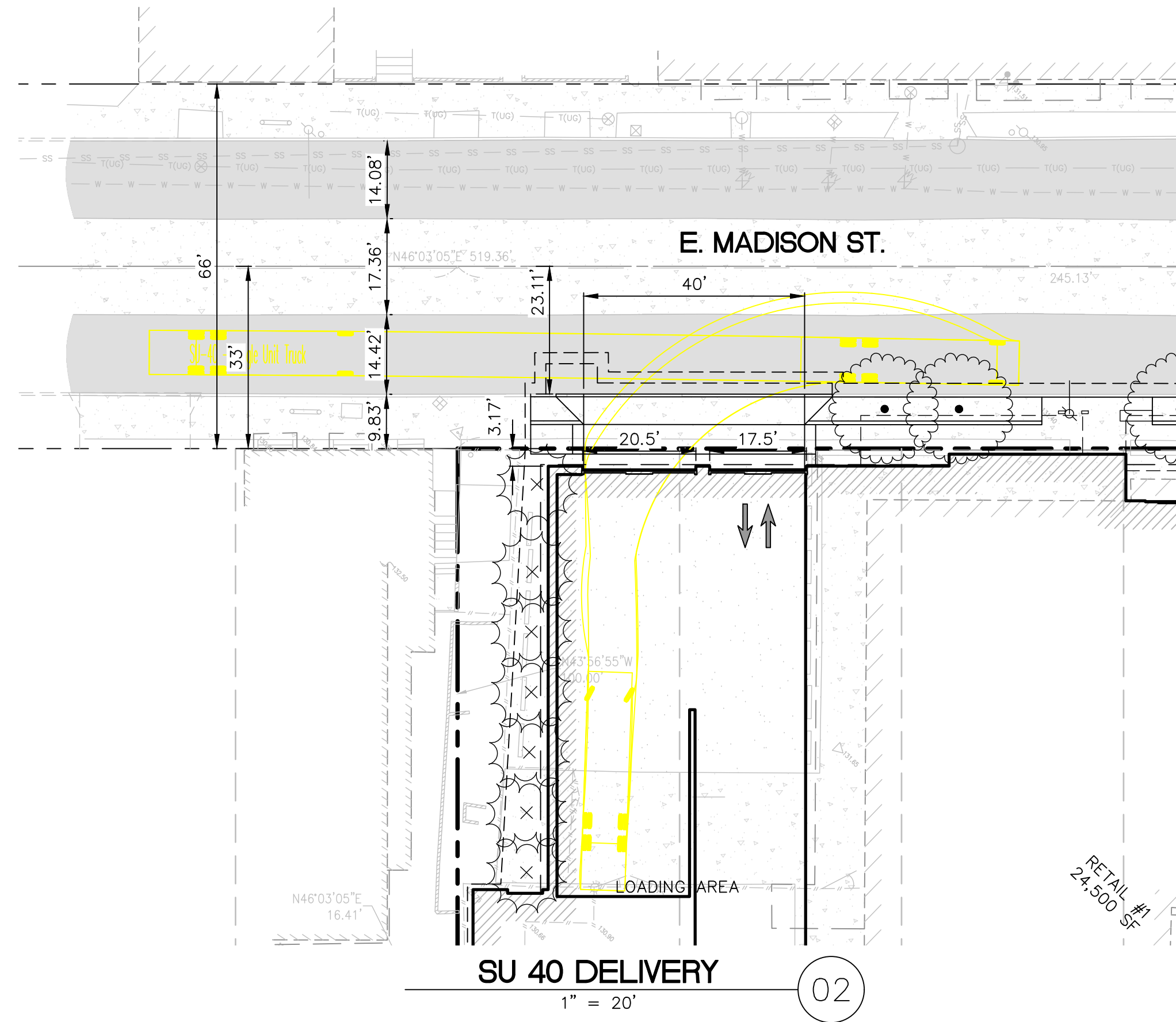
SU-40 - Single Unit Truck
